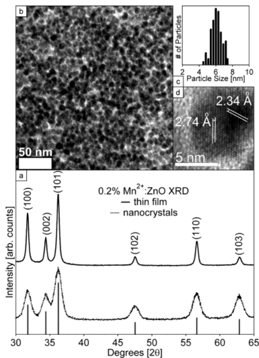
Figure 3. (a) Powder X-ray diffraction data: (---) 0.20% \text{Mn}^{2+}:\text{ZnO} nanocrystals; (—) thin film prepared from the 0.20% \text{Mn}^{2+}:\text{ZnO} nanocrystals. Peak positions for wurtzite ZnO are included for reference. (b) Overview TEM image of 0.20% \text{Mn}^{2+}:\text{ZnO} nanocrystals. (c) Histogram of 100 crystal diameters ( 6.1 \pm 0.7 nm average diameter). (d) High-resolution TEM image of a single nanocrystal showing lattice spacings matching those of ZnO.
