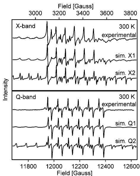
Figure 5. Experimental and simulated 300 K X- and Q-band EPR spectra of colloidal dodecylamine-capped 0.02% Mn 2+ :ZnO nanocrystals in toluene. Simulations with (X1 and Q1) and without (X2 and Q2) \sigma = 2\% D -strain are included.
