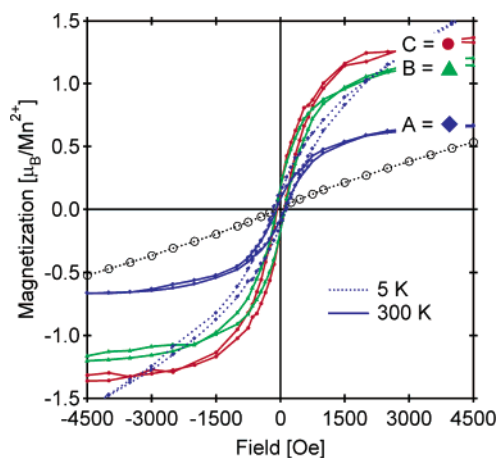
Figure 8. 5 K (···) and 300 K (—) magnetic susceptibilities of 0.20% \text{Mn}^{2+}:\text{ZnO} nanocrystals (○) and thin films (◆, film A; ▲, film B; ●, film C).
