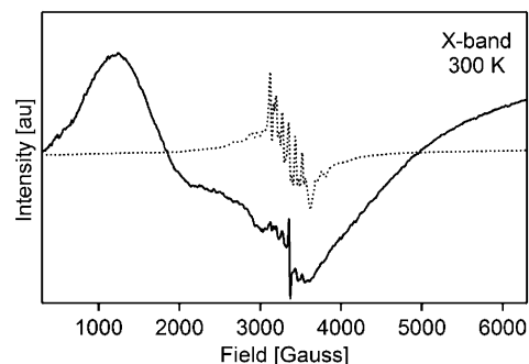
Figure 10. 300 K X-band EPR spectra. (—) Ferromagnetic 0.20% \text{Mn}^{2+}:\text{ZnO} thin film (film A) from Figure 8. (···) The colloids from which film A was prepared, suspended in toluene.
