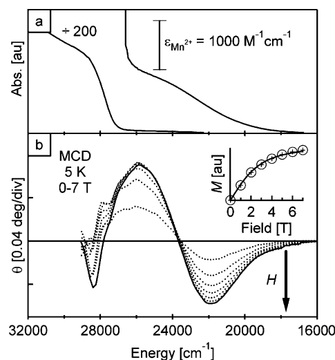
Figure 6. (a) 300 K absorption spectrum of colloidal TOPO-capped 1.1% Mn 2+ :ZnO nanocrystals. (b) Variable-field 5 K MCD spectra of the same nanocrystals, drop-coated onto quartz disks to form frozen solutions. The inset shows the 5 K MCD saturation magnetization probed at 21 900 cm -1 . The solid line shows the S = 5/2 saturation magnetization at 5 K predicted by the Brillouin function (eq 4).
