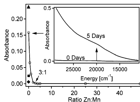
Figure 4. Absorption intensities of various solutions of 0.002 M \text{Mn}(\text{OAc})_2 in DMSO measured at 20\,000\text{ cm}^{-1} after 5 days in air. (○) Solutions with varying ratios of \text{Zn}(\text{OAc})_2 to \text{Mn}(\text{OAc})_2 . (▲) A solution with a 5:1 ratio of \text{Na}(\text{OAc}) to \text{Mn}(\text{OAc})_2 . (■) An anaerobic solution of \text{Mn}(\text{OAc})_2 . (◆) A solution with 0.002 M \text{Mn}(\text{NO}_3)_2 instead of \text{Mn}(\text{OAc})_2 . Inset: Absorption spectra of a DMSO solution of 0.002 M \text{Mn}(\text{OAc})_2 after mixing (0 days) and after 5 days in air.
